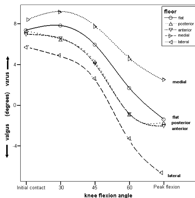
Fig. 2. Coronal plane motion of the knee during landing on level and inclined floors.
